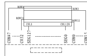
COM&SEG LAYOUT
