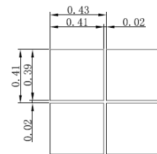
Detail A (20:1)
