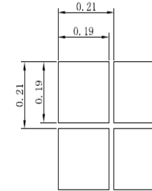
Detail A (30:1)
